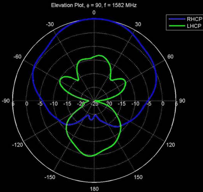
1582 MHz
