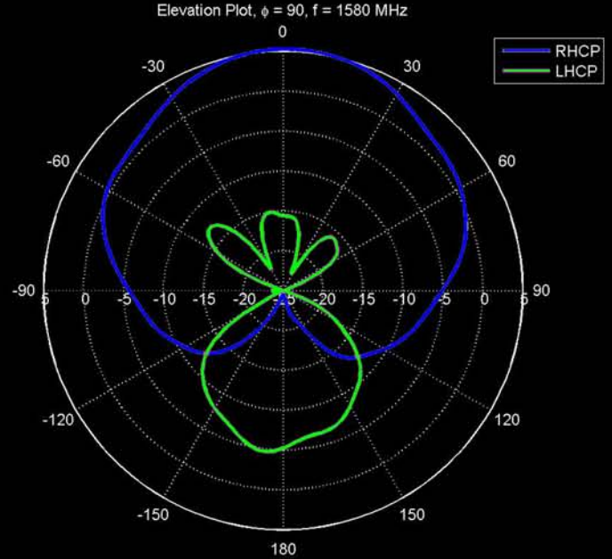
1580 MHz
