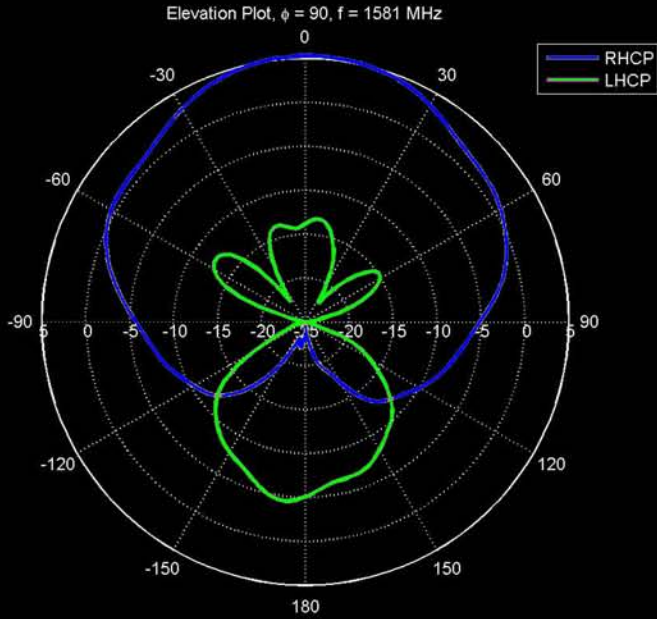
1581 MHz
