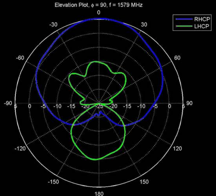
1579 MHz
